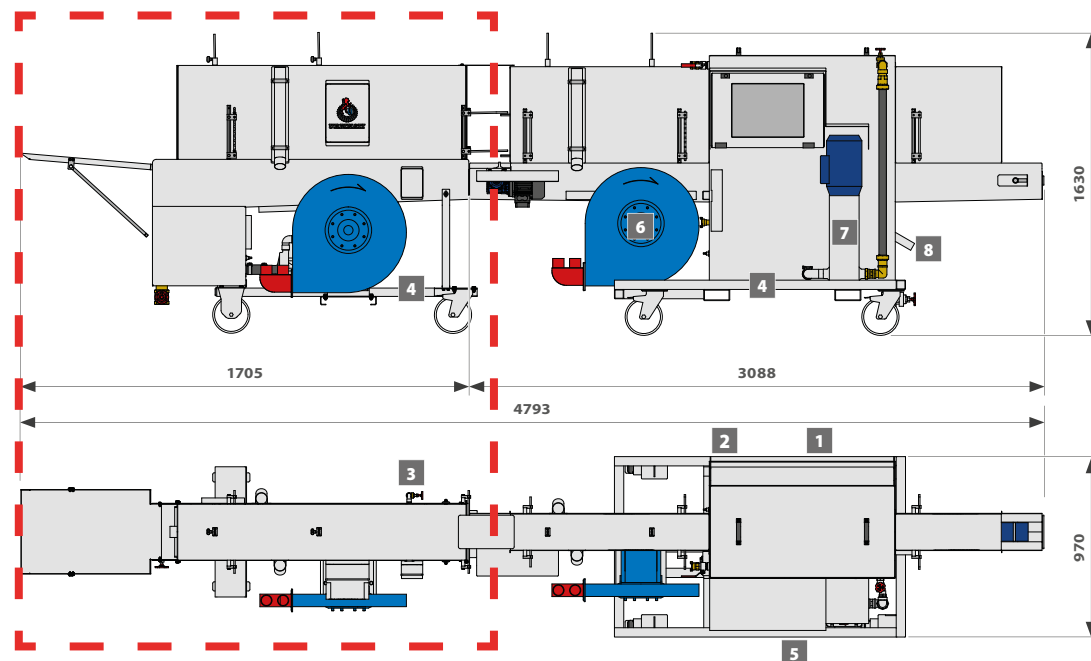
TUNNEL FOR DISINFECTON (accessory)
