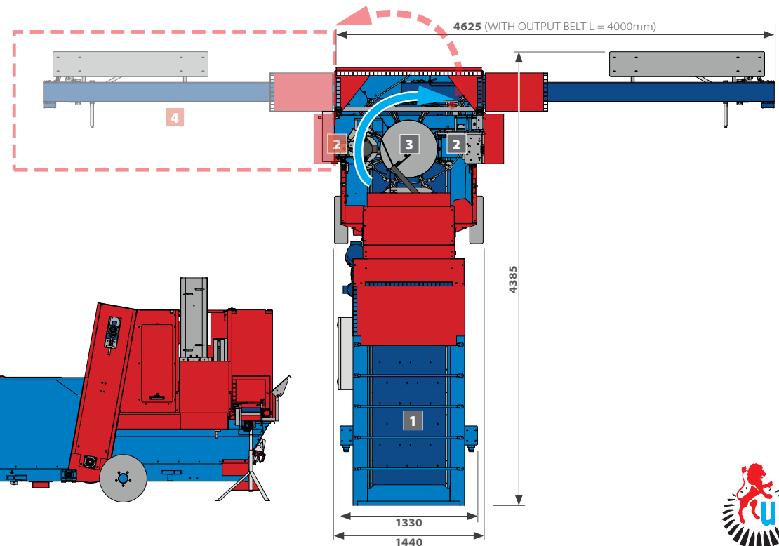
Pots feeding belt, combined with double head for square pots (accessory).
